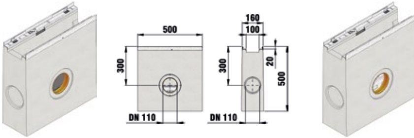
Trash box with composite bucket
